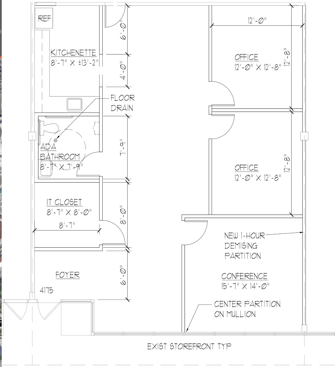
OFFICE SPACE FLOOR PLAN
